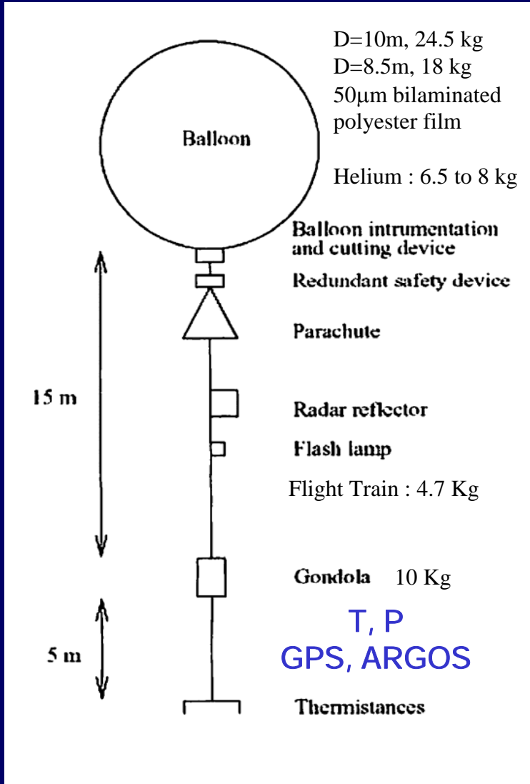
FIG. 4. The flight train configuration during Vorcore.
