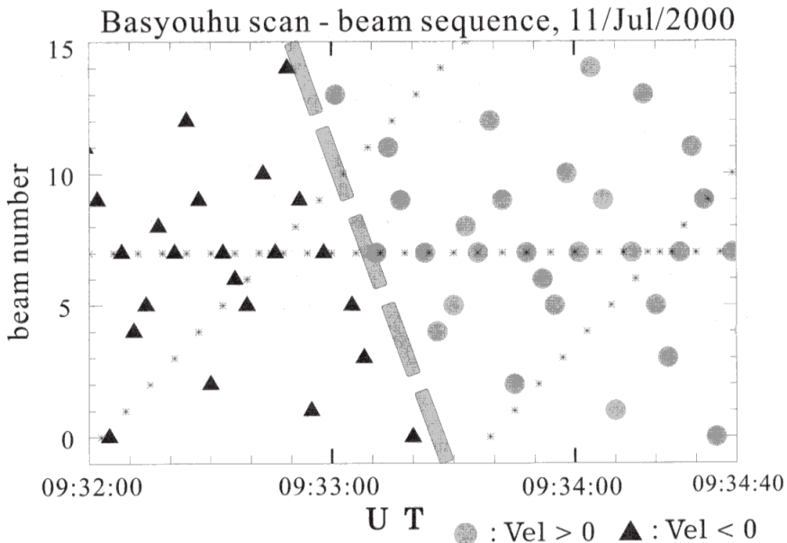
Fig. 4. Line-of-sight velocity change at a range gate of 14 (about 810 km away from the Syowa radar) for all of the observed beams over a period between 0932:00 and 0934:40 UT on July 11, 2000. The horizontal axis is the universal time (UT) and the vertical axis represents the beam number. The triangles represent a negative LOS velocity observation (red-colored region in Fig. 3) and the circles represent a positive LOS velocity observation (blue-colored region). The asterisks show the beam sequence in case of normal global scan with a high time resolution camping beam (7) and an integration period of 3 s. The thick dashed line shows the sharp boundary between the negative velocity region and the positive velocity region.
