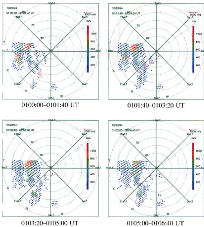
Fig. 5c. Same as Fig. 5a except 0100:00–0106:40 UT.
