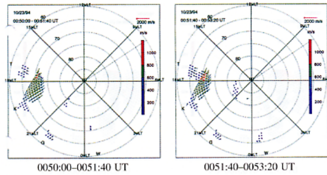
Fig. 5a. Plot of the averaged line-of-sight velocity values obtained from the SuperDARN radars on 23 October 1994, 0046:40–0053:20 UT. The longitude positions (in geomagnetic coordinates) of the contributing radars are indicated by the letters along 60°N contour; T, Saskatoon; K, Kapuskasing; G, Goose Bay; W, Stokkseyri.
