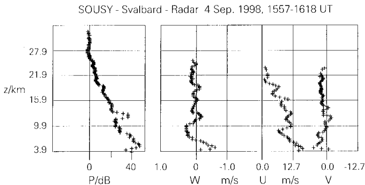
Fig. 5. Height profiles of signal power P (normalized to the noise level at 0 dB), radial velocity in the vertical beam ( W ), and zonal ( U ) and meridional ( V ) wind velocity, measured with the SSR on 4 September 1998 at 1557–1618 UT.
