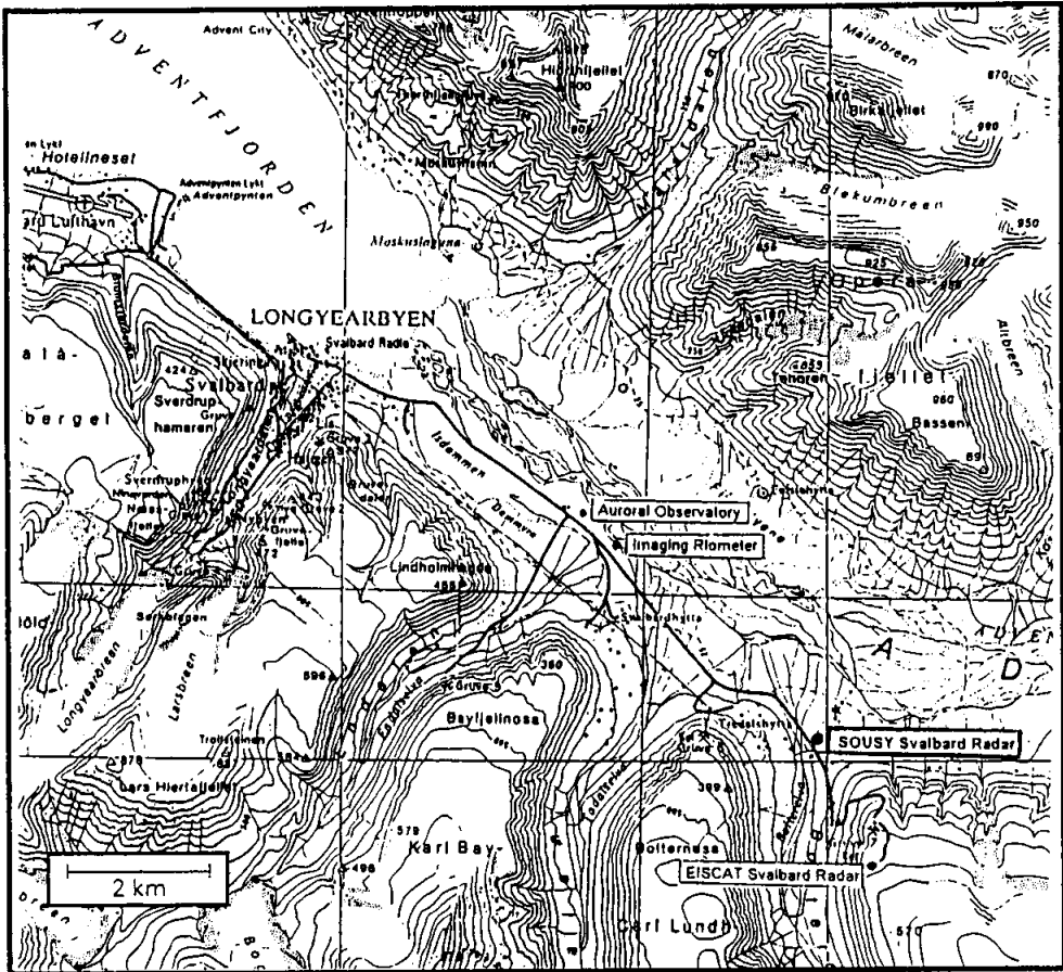
Fig. 1. The locations of facilities for middle and upper atmosphere research in the vicinity of Longyearbyen Svalbard. The EISCAT Svalbard Radar (ESR) is close to the top and the SOUSY Svalbard Radar (SSR) at the foot of the mountain of coalmine 7. The imaging riometer (IRIS) is close to the Auroral Observatory, where also the OH spectrometer is located.
