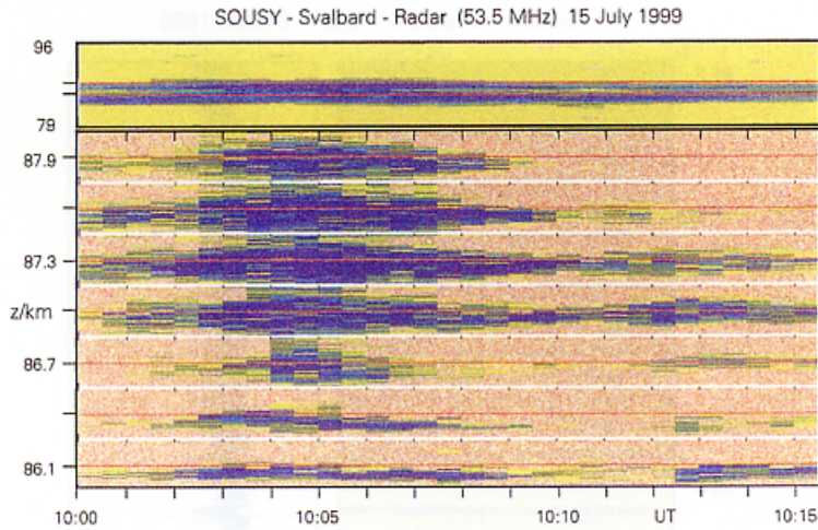
Fig. 10. Same as Fig. 8 but dynamic spectra between 85.2 km and 89.7 km with different time-scale to match to the time scale of Fig. 9, which was recorded simultaneously with the ESR on 15 July 1999.
