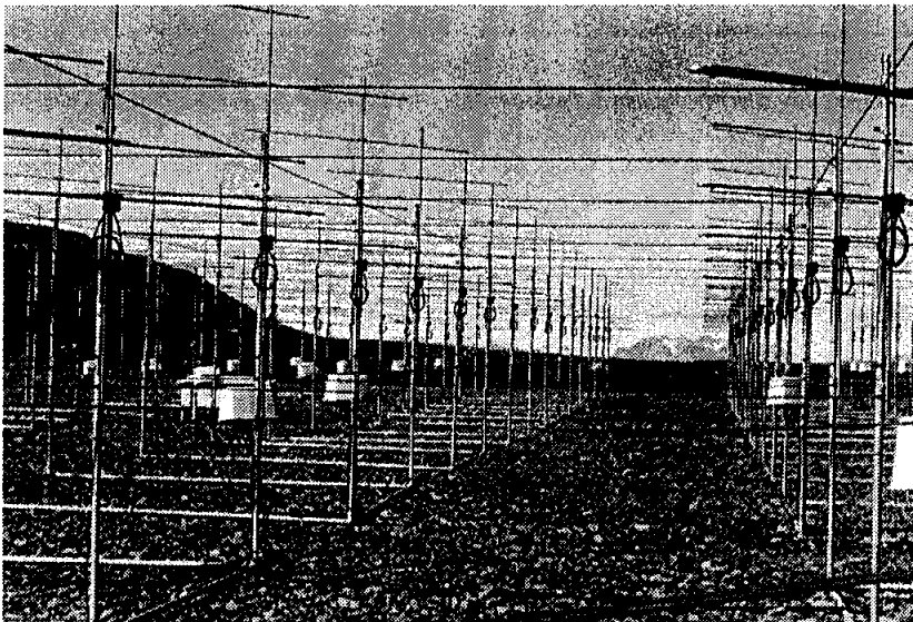
Fig. 2. Part of the antenna array of the SOUSY Svalbard Radar in Adventdalen/Bolterdalen near Longyearbyen.
