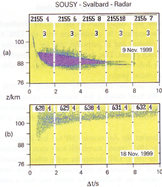
Fig. 12. a) Meteor echo detected with the SSR on 9 November 1999 between 2155:04 and 2155:10 UT with the antenna beam pointing at 5^\circ zenith angle into SW direction.
