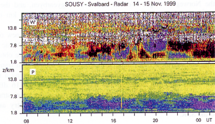
Fig. 6. Height-time-intensity plots of received normalized power P (lower panel) and radial velocity W in the vertical beam direction (upper panel), recorded with the SSR between 0739:18 UT on 14 November 1999 and 0135:05 UT on 15 November 1999. The velocity scale is between -1 \text{ m s}^{-1} (black) and +1 \text{ m s}^{-1} (magenta); velocity estimates are affected by noise below and above the tropopause. The power is normalized to the noise level and its scale is between 0 dB (noise level; yellow) and 20 dB (magenta). Transmission was with the full 356-Yagi antenna and reception was with 4 Yagis only.
