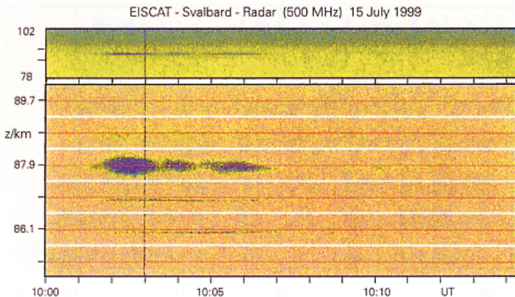
Fig. 9. Polar Mesosphere Summer Echoes recorded with the ESR (antenna pointing 30^\circ zenith angle at 135^\circ azimuth) on 15 July 1999. The upper panel shows the height-time-intensity plot between 78.3 km and 101.7 km altitude. The lower six panels show the dynamic spectra for the range gates between 85.2 km and 89.7 km. The Doppler velocity limits in this display are \pm 27.8 \text{ m s}^{-1} ; zero velocity is indicated by the red line.
