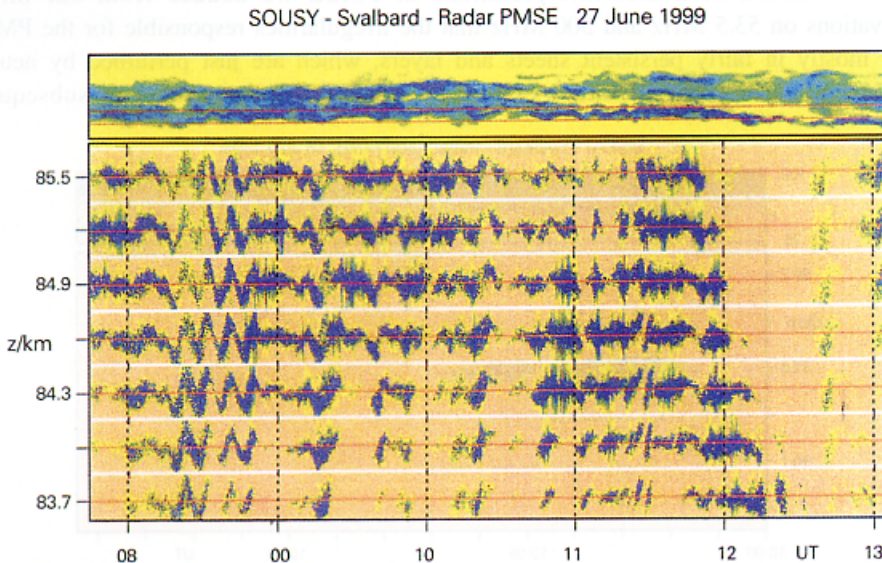
Fig. 8. Polar Mesosphere Summer Echoes recorded with the SSR (vertical beam) between 0745:03 UT and 1305:25 UT on 27 June 1999. The upper panel shows the height-time-intensity plot between 79.2 km and 95.7 km altitude, and the lower 7 panels the dynamic spectra of altitude gates 83.7 km and 85.5 km. The Doppler frequency limits in this display are \pm 2.8 Hz, corresponding to a radial velocity of \pm 7.9 m s -1 . The center red line indicates zero velocity.
