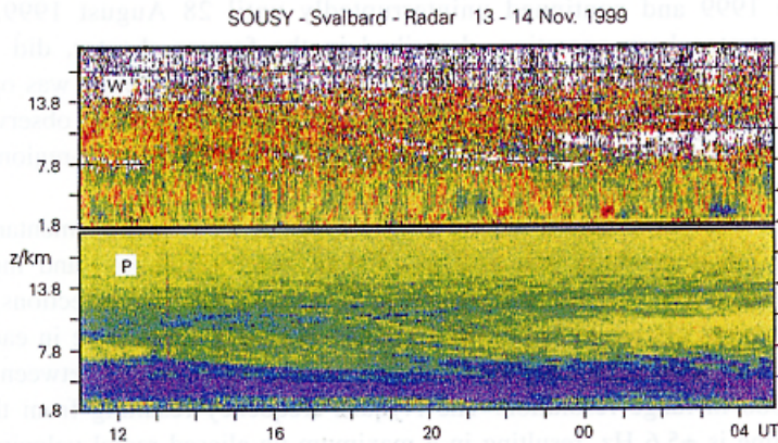
Fig. 7. Same as Fig. 6, but between 1100:38 UT on 13 November 1999 and 0456:24 UT on 14 November 1999.
