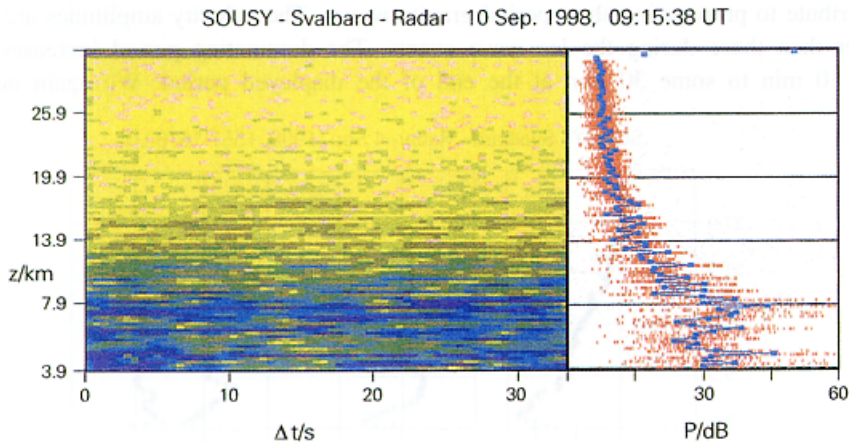
Fig. 4. Quicklook example of first SSR measurements of the troposphere and stratosphere using the full antenna for transmission and reception. Left-hand: Height-time-intensity plot, covering a short period of 32 s, showing thin layers in the troposphere and lower stratosphere. Right-hand: Scatter plot of normalized power P (signal + noise). The antenna was pointing into vertical direction.
