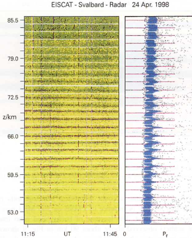
Fig. 11. Incoherent scatter echoes observed with the ESR on 24 April 1998 between 1115 UT and 1145 UT with antenna beam pointing into direction of the Earth's magnetic field. The Doppler velocity limits are \pm 55.5 \text{ m s}^{-1} ; the tick marks on the height axis and the red lines in the right-hand panel correspond to zero Doppler velocity in the corresponding range gate. The left-hand panel shows the dynamic spectra and the right-hand panel the distributions of relative power during the observing period.
