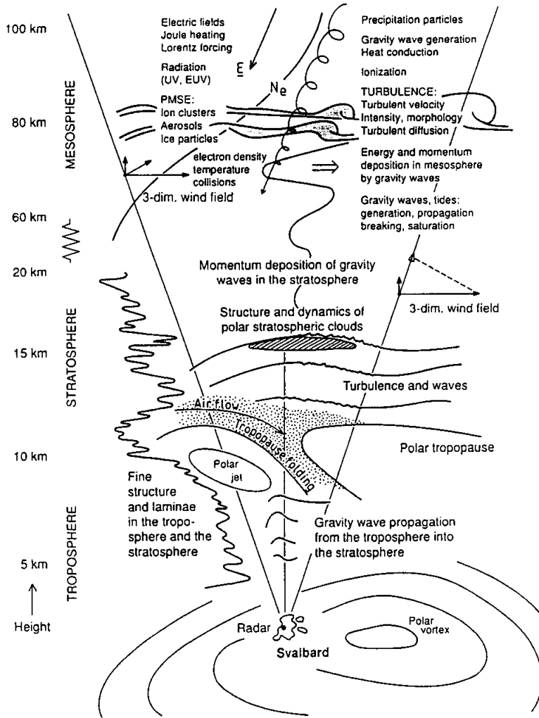
Fig. 3. Processes in the polar mesosphere, stratosphere and troposphere, which can be studied by an MST VHF radar (SSR). The lower thermospheric and ionospheric processes are measured by incoherent scatter radar (ESR); from Röttger and Tsuda (1995).
