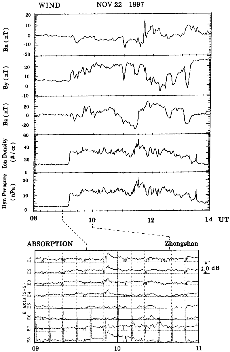
Fig. 6. Variation in the B_x , B_y , and B_z components of the IMF, ion density, and ion dynamic pressure of the solar wind determined from the WIND satellite during 0800–1400 UT on November 22, 1997 (upper panel). Variation in the ionospheric absorption in the east-west beams near the zenith during 0900–1100 UT at ZHS (lower panel). Dashed lines between the upper and lower panels show the 38-min delay.
