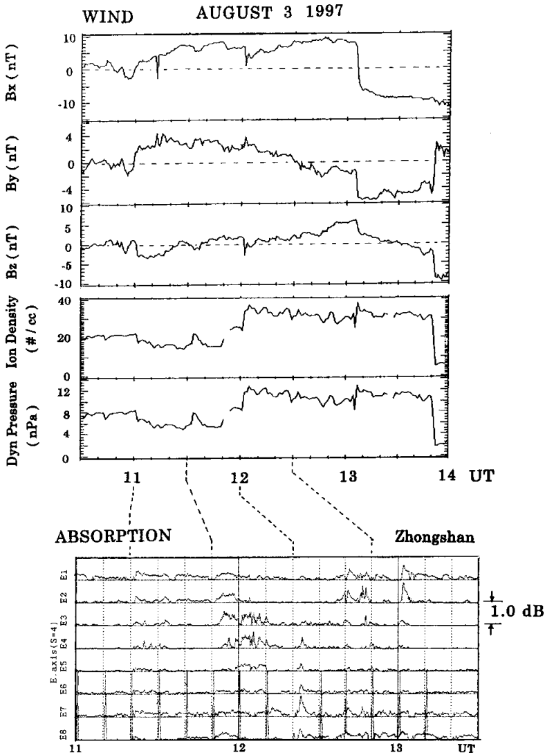
Fig. 3. Variation in the B_x , B_y , and B_z components of the IMF, ion density, and ion dynamic pressure of the solar wind determined from the WIND satellite during 1030–1400 UT on August 3, 1997 (upper panel). Variation in the ionospheric absorption in the east-west beams near the zenith during 1100–1330 UT at ZHS (lower panel). The dashed lines between the upper and lower panels show the 20-min delay.
