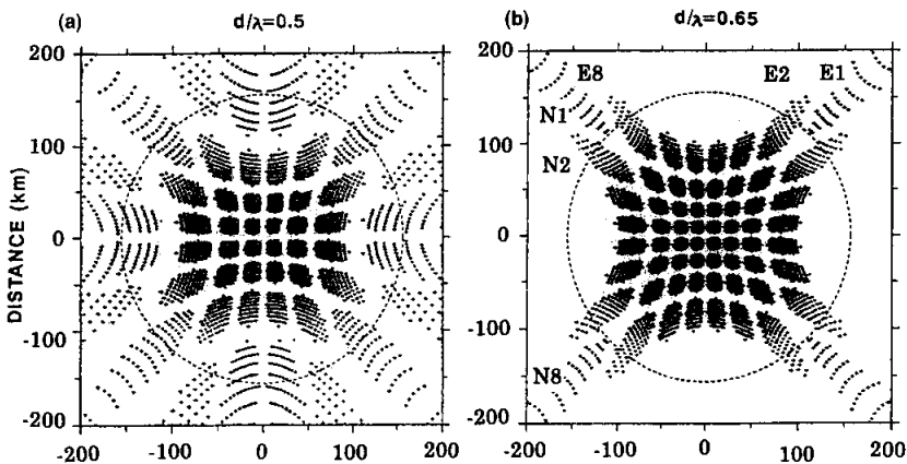
Fig. 1. The projection of a half-power width of the 64 antenna-beams onto an ionospheric absorption altitude of 90 km. The patterns are shown for (a) 0.5-wavelength spacing (Zhongshan station) and (b) 0.65-wavelength spacing (Ny-Ålesund station) (after Yamagishi et al. , 1992). The beam numbers are assigned for north-south and east-west cross sections in pattern (b).
