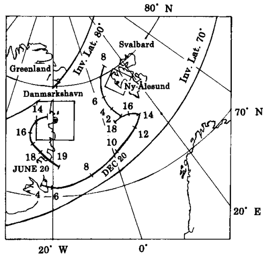
Fig. 2. The IRIS FOV at Danmarkshavn and Ny-Ålesund with the invariant latitudes on a map of the European arctic. Daily variation in the conjugate points for Zhongshan is drawn for the northern summer and winter solstices, based on calculations using the 1996 Tsyganenko model (modified after Yamagishi et al. , 1998).
