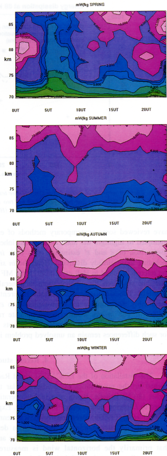
Fig. 6. Kinetic energy dissipation rate (method of Hall, 1997) as a function of time of day, height and season, in order to illustrate tidal dependence (Hall, 1998). Contours are in \text{mWkg}^{-1} .
