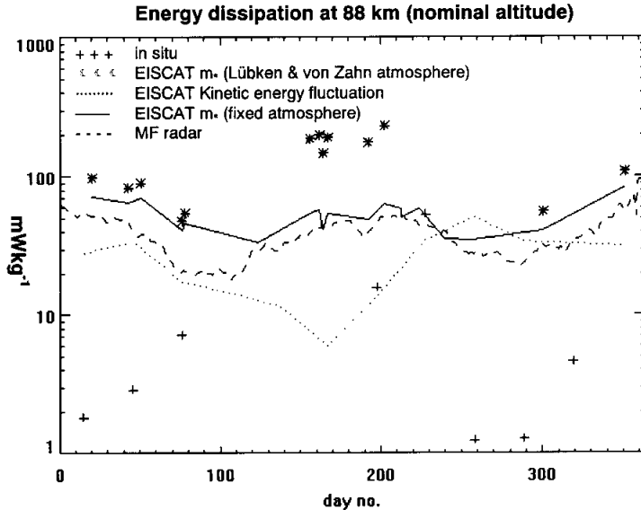
Fig. 7. Seasonal variation of energy dissipation rate (see text for explanation of the different definitions. The EISCAT m_{-} method has been performed for two different model atmospheres, to illustrate the sensitivity to scale height and buoyancy frequency (Hall and Hoppe, 1998).
