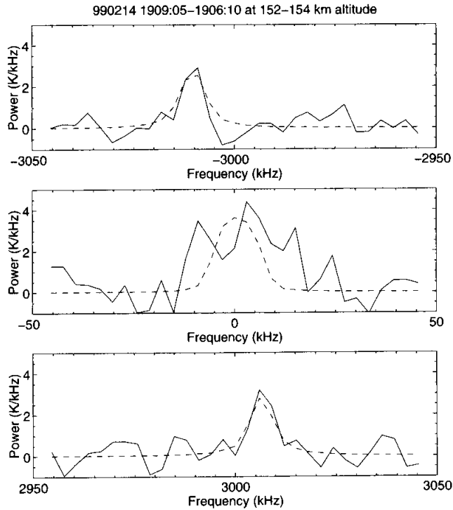
Fig. 15. Measured spectra of the both plasma lines and the ion line and the best 7-parameter fit of the theoretical spectrum. The parameters fitted were N_e=9.7 \cdot 10^{10} \text{ m}^{-3} , T_e=631 \text{ K} , T_i=697 \text{ K} , v_i=-100 \text{ ms}^{-1} , v_e=657 \text{ ms}^{-1} and a suprathermal distribution with n_e=0.8 \cdot 10^9 \text{ m}^{-3} and T=11 \text{ eV} .
