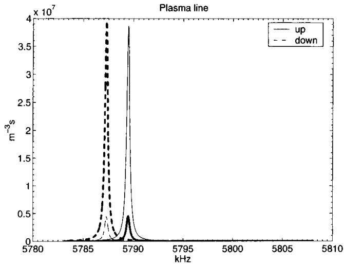
Fig. 10. The plasma lines based on an upgoing (thick line) and downgoing 10 eV beam of suprathermal electrons at a current of 1 \mu Am^{-2} and temperature of 5 eV. The thermal parameters are the same as in Fig. 8
