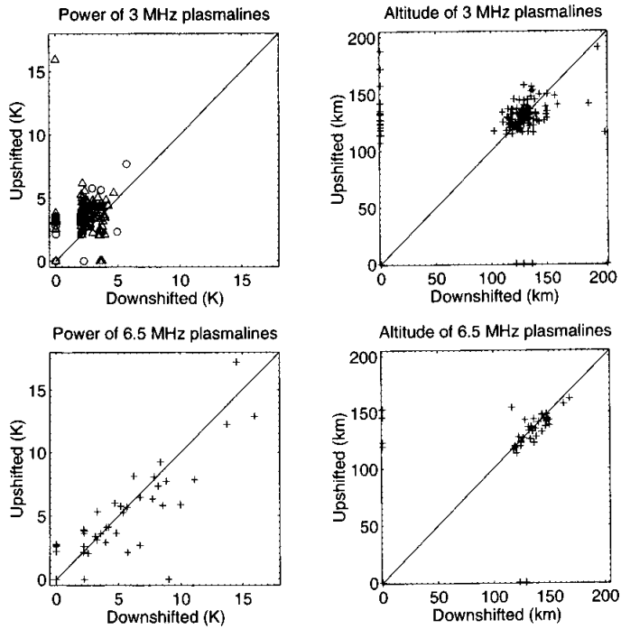
Fig. 13. Scatter plots of power and altitude for the two simultaneously measured up and downshifted lines at 3 and 6.5 MHz. The triangles and circles for the power of the 3 MHz case, in the upper left, show lines detected before and after magnetic midnight respectively — no difference can be seen.
