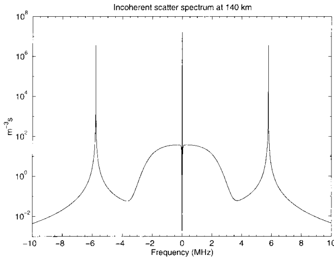
Fig. 8. The wide frequency incoherent scatter spectrum. The parameters used: N_e=4 \cdot 10^{11} \text{ m}^{-3} , T_e=700 \text{ K} , T_i=600 \text{ K} , v_i=v_e=0 \text{ ms}^{-1} and collision frequencies \nu_e and \nu_i using the MSIS90e model (Hedin, 1991) for 140 km altitude. Logarithmic scale for the strength is used to be able to emphasise the different lines of the spectrum.
