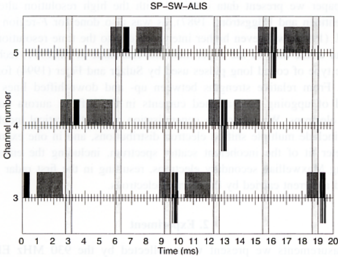
Fig. 1. Transmission (black) and reception (dark gray) scheme for part of SP-SW-ALIS. A 16-bit alternating code, 22 \mu\text{s} bits, is cycled over 3 frequencies. The interscan period is 9 ms and the total cycle takes 300 ms. The plasma line channels were set to sample the same range extent as the ion lines.
