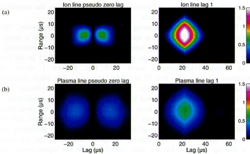
Fig. 2. Range-lag ambiguity function for the first two lags, a) ion line and b) plasma line. The range, given in \mu\text{s} , can be converted to km with multiplication of 0.15. The differences between the ion and plasma line ambiguity functions are due to the use of different receiver filters.
