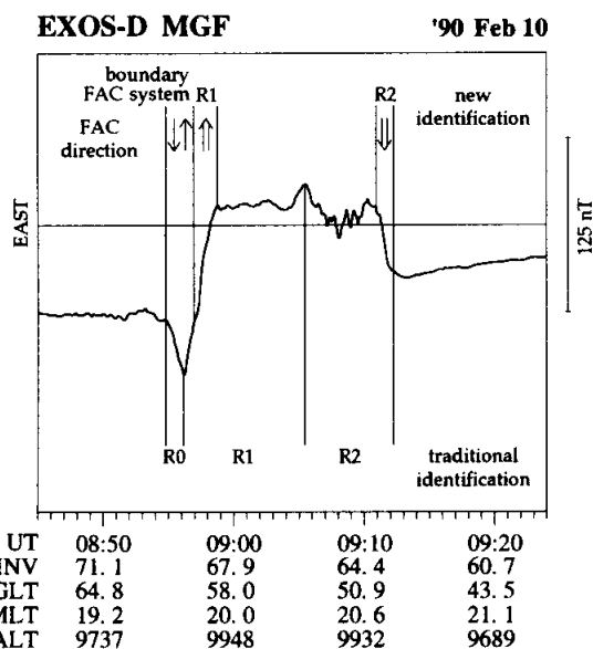
Fig. 3. East-west component of magnetic field perturbation obtained from the EXOS-D observations on February 10, 1990. According to our definitions of the local and global FACs (see text), the regions of the boundary FAC system, the region 1 FAC and the region 2 FAC are indicated above the curve of magnetic perturbation. (The boundary FAC system may partly overlap with the region 1 system. In this figure, for simplicity, we assume that there is a single interface between them.) Below the magnetic perturbation curve, illustrated is the traditional identification of the region 0, region 1 and region 2 FAC zones.
