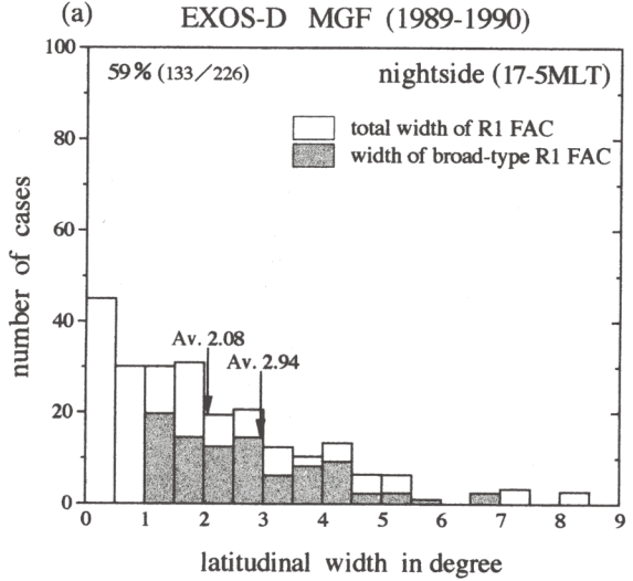
Fig. 7. (a) Numbers of the region 1 FAC systems in the 17-5 MLT range versus the (total) latitudinal width of the system. The gray-shaded histogram shows the numbers of the broad-type region 1 FAC systems (without a T-structure) versus the system width. (b) Same as (a), but for each two-hour MLT sector. Two separate histograms in the 23-25 (=01) MLT sector are shown for the evening and morning types of the region 1 current system. In the upper left corner of each histogram in (a) and (b), the percentage of the number of the T-structures relative to the whole number of the region 1 systems is indicated together with these two numbers in a fraction.
