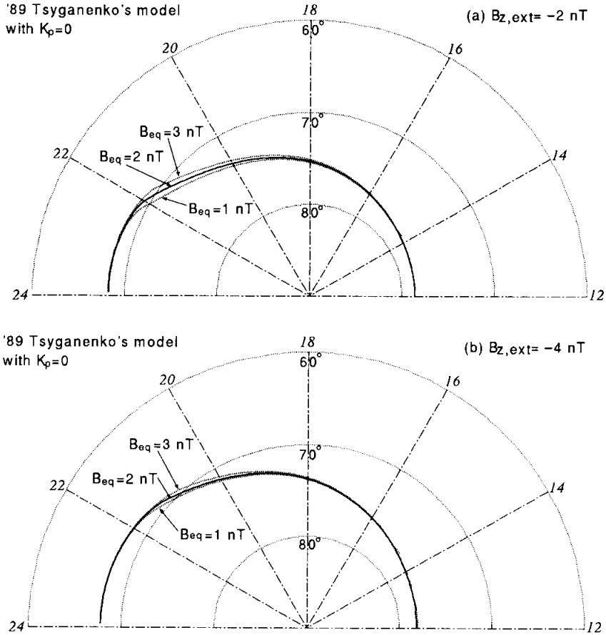
Fig. 6. Ionospheric footprints of the B_{eq} = 1 nT, 2 nT and 3 nT lines for (a) B_{z,ext} = -2 nT and (b) B_{z,ext} = -4 nT, both for K_p = 0 .
