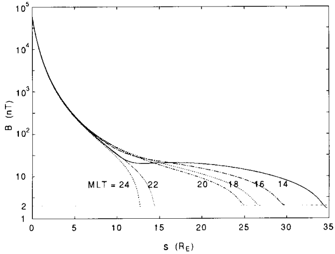
Fig. A3. Magnetic field strengths varying along the field lines depicted in Fig. A1, where s is the field-aligned distance from the Earth surface.
