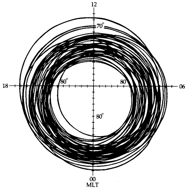
Fig. 5. Auroral circles fitted to the poleward boundary of the auroral belt photographed from the DMSP satellites, a reproduction of Fig. 6 in MENG et al. (1977). The centers of the auroral circles were found to be concentrated within a circular area of 3^\circ radius centered at \sim 4.2^\circ away from the geomagnetic pole along the 0010 MLT (nearly midnight) meridian (see Fig. 5a in their paper).
