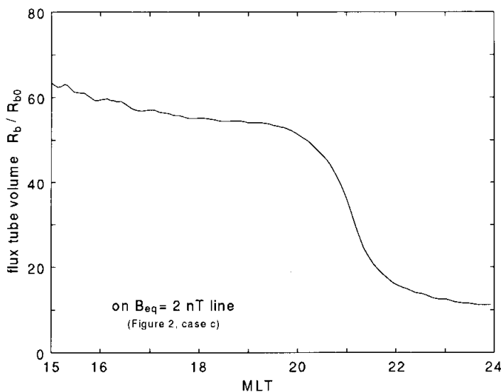
Fig. 8. Flux tube volume R_b/R_{b0} varying along the B_{eq} = 2 nT line (in Fig. 2, case c).
