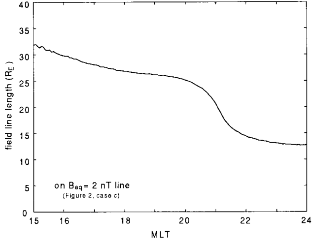
Fig. A2. Total length of the field line (between the ionosphere and the equator) on the B_{eq} = 2 nT line (in Fig. 2, case c) plotted against (dusk-side) MLT.
