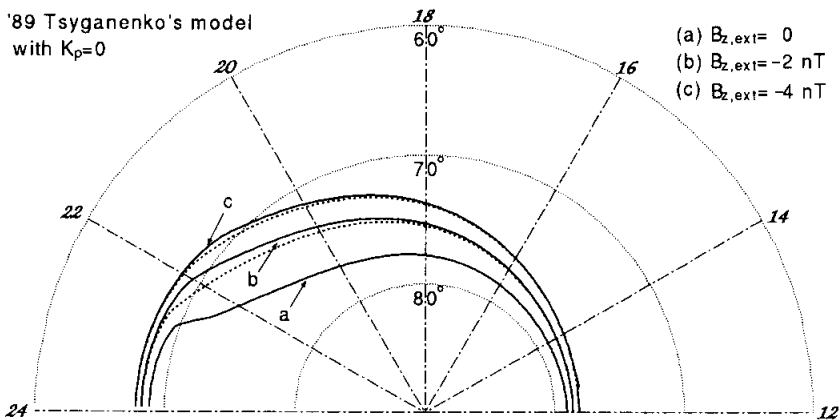
Fig. 2. Solid lines show the ionospheric footprints of the B_{eq}=2nT lines in Fig. 1, for (a) B_{z,ext}=0 , (b) B_{z,ext}=-2nT and (c) B_{z,ext}=-4nT , and dotted lines show the open-closed boundaries in cases of (b) and (c). Dial of MLT (12-24) and lines of 60^\circ, 70^\circ and 80^\circ magnetic latitudes are indicated.
