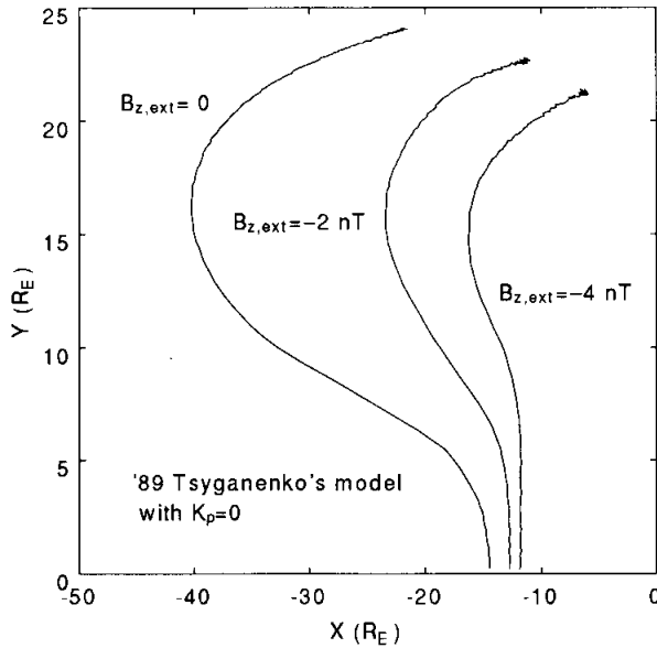
Fig. 1. Equicontours of ' B=B_{eq}=2nT ' in the X - Y plane, for three cases of B_{z,ext}=0, -2 and -4nT . The local time ranges of the contours are such that their (field-aligned) projections to the ionosphere (see Fig. 2) range between 24 and 15 MLT. Coordinates X and Y are in units of the Earth radius, R_E .
