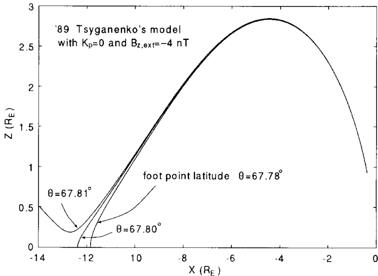
Fig. 3. Field lines near the separatrix in the Z - X plane, for the case of B_{Z, \text{ext}} = -4 nT.
