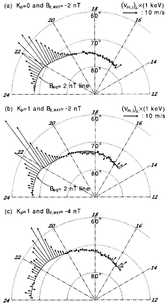
Fig. 10. Same format as in Fig. 9, but for (a) K_p=0 and B_{Z,ext} = -2 nT, (b) K_p = 1 and B_{Z,ext} = -2 nT, (c) K_p = 1 and B_{Z,ext} = -4 nT
