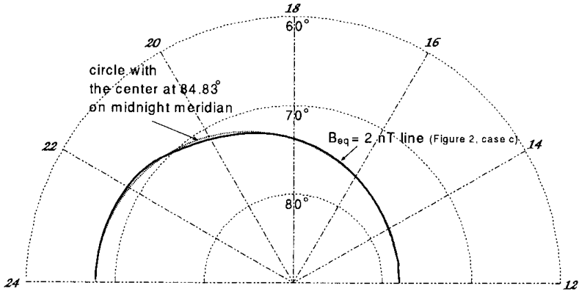
Fig. 4. Comparison of the B_{eq}=2\text{ nT} line with a typical auroral circle with the center at a latitude of about 85^\circ on the midnight meridian.
