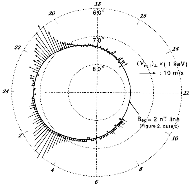
Fig. 9. Perpendicular (to the B_{\text{eq}} = 2 \text{ nT} line) component of the average magnetic drift velocity, (\bar{\nu}_{m,i})_{\perp} \times (1 \text{ keV}) , projected to the ionosphere, for an ion fluid with isotropic pressure and an average energy of 1 \text{ keV} is plotted along the B_{\text{eq}} = 2 \text{ nT} line (in Fig. 2, case c). (Over the interval of 17–15 MLT, (\bar{\nu}_{m,i})_{\perp} changes irregularly and sometimes its direction is reversed, i.e., directed poleward, although in reality (\bar{\nu}_{m,i})_{\perp} must be invariably directed equatorward in the case of this figure. The cause of such irregularities in (\bar{\nu}_{m,i})_{\perp} is explained as follows: Basically, within a limited computational time it is difficult to find (for any local time) such a field line as having B_{\text{eq}} extremely close to a given value of 2 \text{ nT} . On the field lines actually identified as those on the B_{\text{eq}} = 2 \text{ nT} , the values of B_{\text{eq}} can deviate, at most 5%, from 2 \text{ nT} . Irregular deviation (from 2 \text{ nT} ) of B_{\text{eq}} causes such irregularities in R_b as shown in Fig. 8, leading to irregularities in (\bar{\nu}_{m,i})_{\perp} .)
