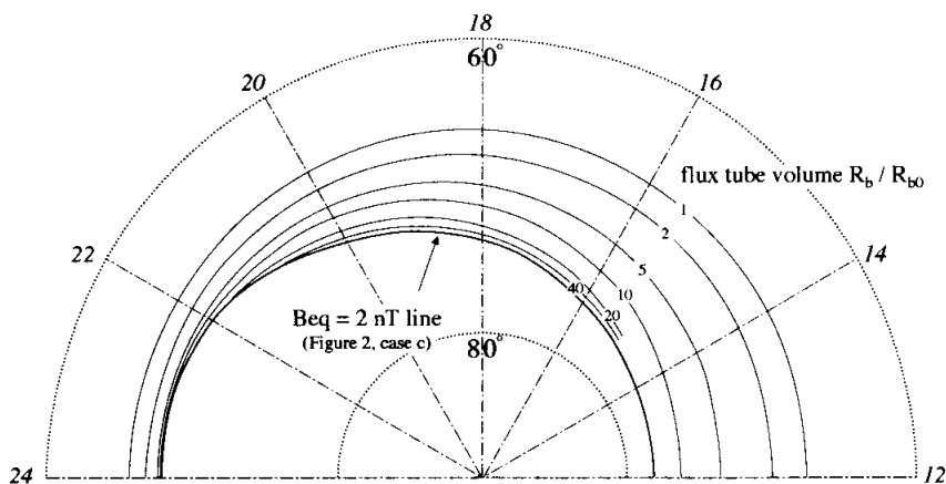
Fig. 7. Equicontours of the flux tube volume R_b , normalized by R_{b0} (for their definitions, see text), on the ionospheric plane. Superposed is the B_{eq} = 2 nT line (in Fig. 2, case c).
