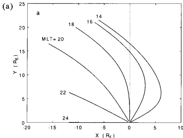
Fig. A1. Projections to, (a) the X - Y plane, (b) the Y - Z plane, and (c) the X - Z plane, of the field lines with ionospheric foot points at various local times on the B_{\text{eq}} = 2 nT line (in Fig. 2, case c).
