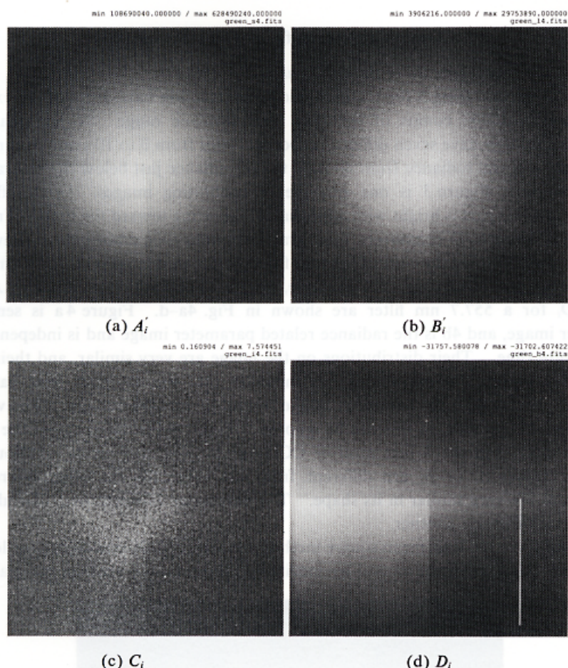
Fig. 4. The parameter image of the absolute calibration (557.7 nm).
