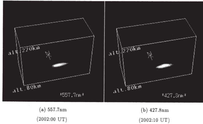
Fig. 7. Visualization of the reconstructed emission rate.
