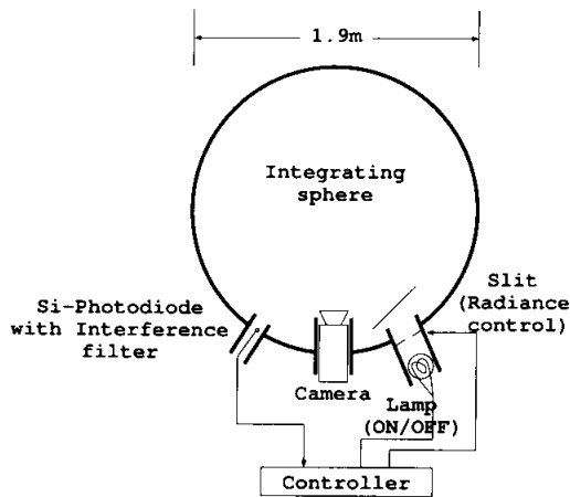
Fig. 2. The integrating sphere calibration standard (OL 462).
