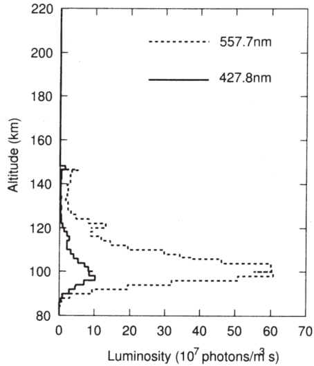
Fig. 8. Profiles of the reconstructed emission rate.
