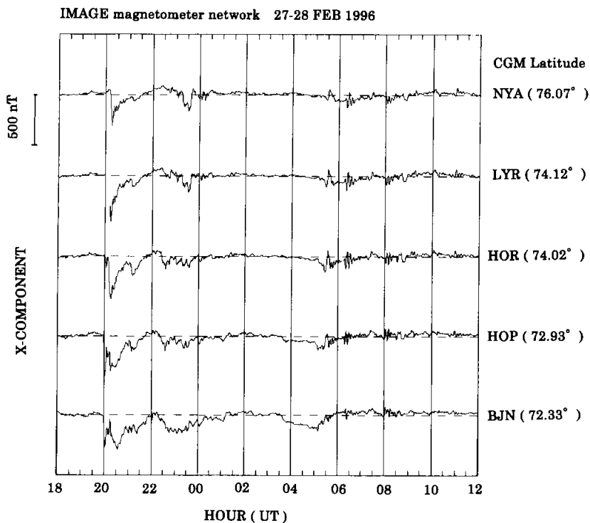
Fig. 5. Time variations in the geomagnetic X-components at Svalbard stations in the IMAGE magnetometer network. The name and the geomagnetic latitude of the stations are noted at the right side.
