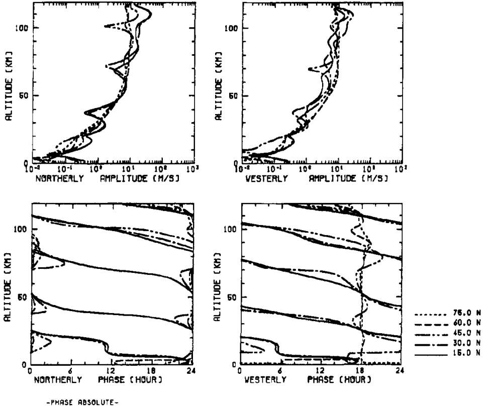
Fig. 3. Numerical profiles of the northerly (left) and westerly (right) components of diurnal tide for the June solstice wind condition by the ATM2 modeling. Latitudes are 15^\circ (solid), 30^\circ (dashed-dot), 45^\circ (dashed-double-dot), 60^\circ (dashed) and 75^\circ (dotted) in the Northern Hemisphere.
