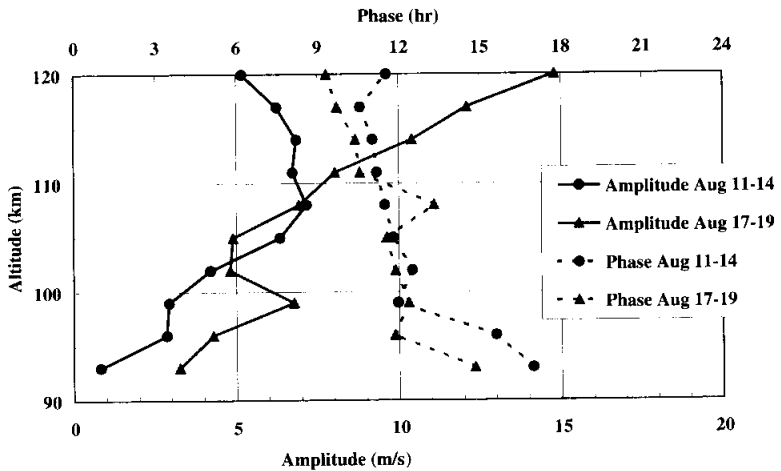
Fig. 2. Altitude profiles of the amplitude (solid line) and phase (dashed line) of 24-hr component for the Test (circle) and CP (triangle) periods.
