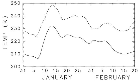
Fig. 1. Time series of the zonal mean temperature at 80^{\circ}\text{N} of 30 km (solid line) and 40 km (dotted line). Units are K.
