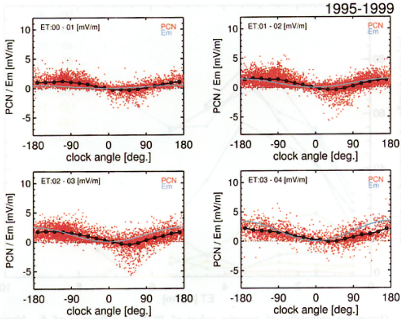
Fig. 3a. Scatter plots of IMF clock angle vs PCN for four ranges of E_T , 00–01 mV/m (top left), 01–02 mV/m (top right), 02–03 mV/m (bottom left), and 03–04 mV/m (bottom right). The black lines with filled circles show the average values of PCN. The blue lines show the calculated merging electric field ( E_m ).
